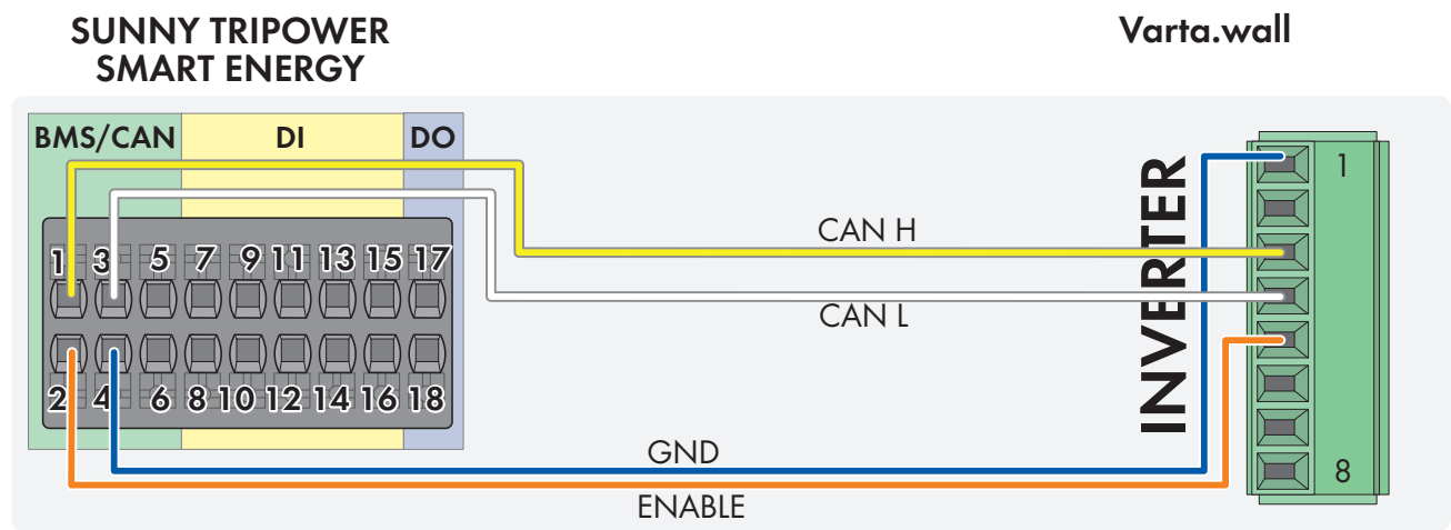
Figure 6: Sunny Tripower Smart Energy with Varta.wall. If an installation cable is not used, the individual cable ends must be provided with a 12 mm long bootlace ferrule.
