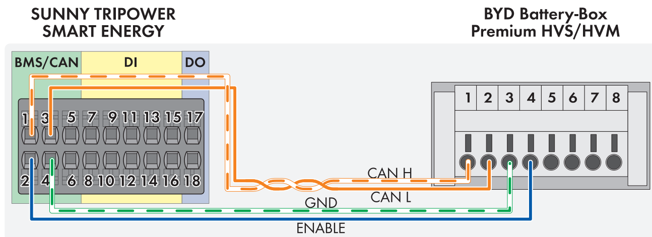
Figure 2: Cabling plan in accordance with TIA-568B: Sunny Tripower Smart Energy with BYD Battery-Box Premium HVM/HVS when using an installation cable.
