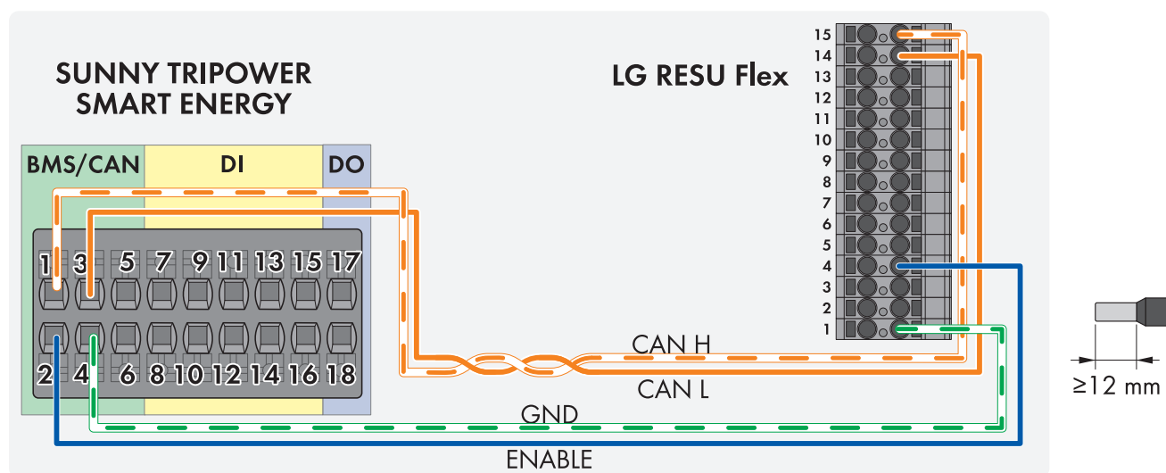
Figure 4: Cabling plan for Sunny Tripower Smart Energy with LG RESU FLEX with installation cable. If an installation cable is not used, the individual cable ends must be provided with a 12 mm long bootlace ferrule.
