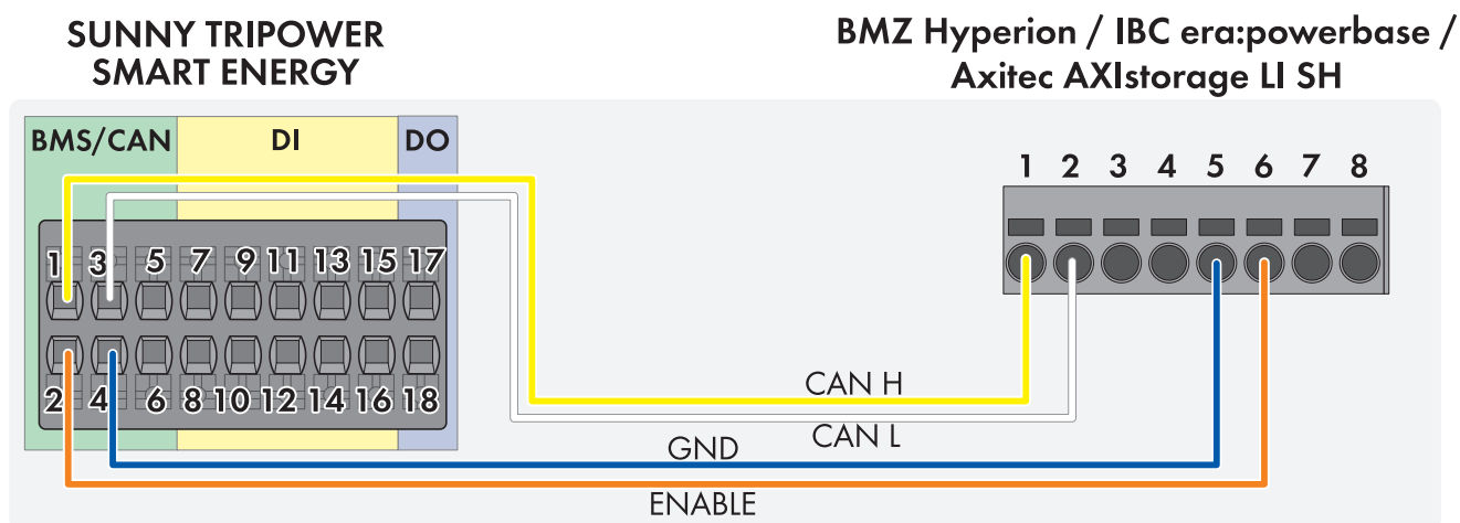
Figure 5: Sunny Tripower Smart Energy with BMZ Hyperion, AXITEC AXIstorage, IBC era:powerbase when using the communication cable provided by the battery manufacturer.
